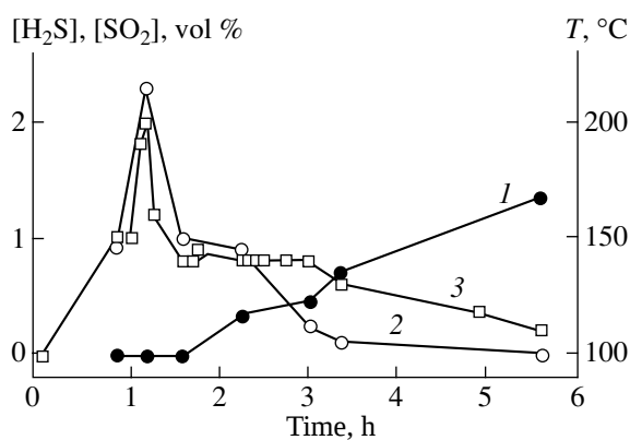
Fig. 2. Plots of the (1) H_2S concentration, (2) SO_2 concentration, and (3) reaction temperature vs. reaction time at an H_2S concentration in the initial gas mixture of 2 vol %, an O_2/H_2S ratio of 5, and a contact time of 0.2 s. Temperature of the initial gas mixture 100^\circ\text{C} .
