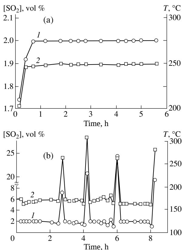
Fig. 1. Plots of the (1) \text{SO}_2 concentration and (2) reaction temperature vs. reaction time at an \text{H}_2\text{S} concentration in the initial gas mixture of 2 vol %, an \text{O}_2/\text{H}_2\text{S} ratio of 5, and a contact time of 0.2 s. Temperature of the initial gas mixture: (a) 203 and (b) 130°C.
