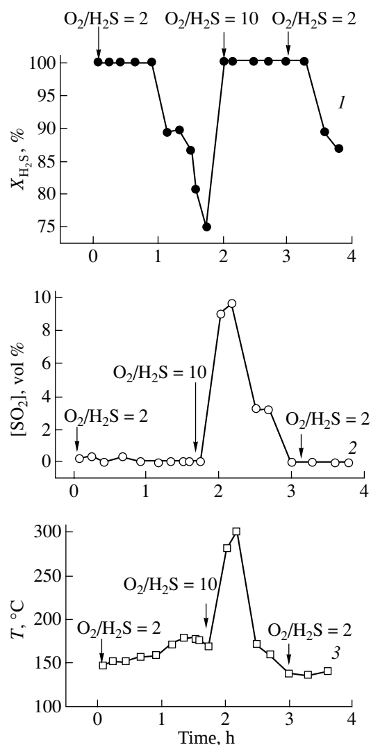
Fig. 4. Plots of the (1) \text{H}_2\text{S} conversion ( X_{\text{H}_2\text{S}} ), (2) \text{SO}_2 concentration, and (3) reaction temperature vs. reaction time at an \text{H}_2\text{S} concentration in the initial gas mixture of 2 vol %, a temperature of the initial gas mixture of 145^\circ\text{C} , and a contact time of 0.2 s. The \text{O}_2/\text{H}_2\text{S} molar ratio changed during the reaction.
