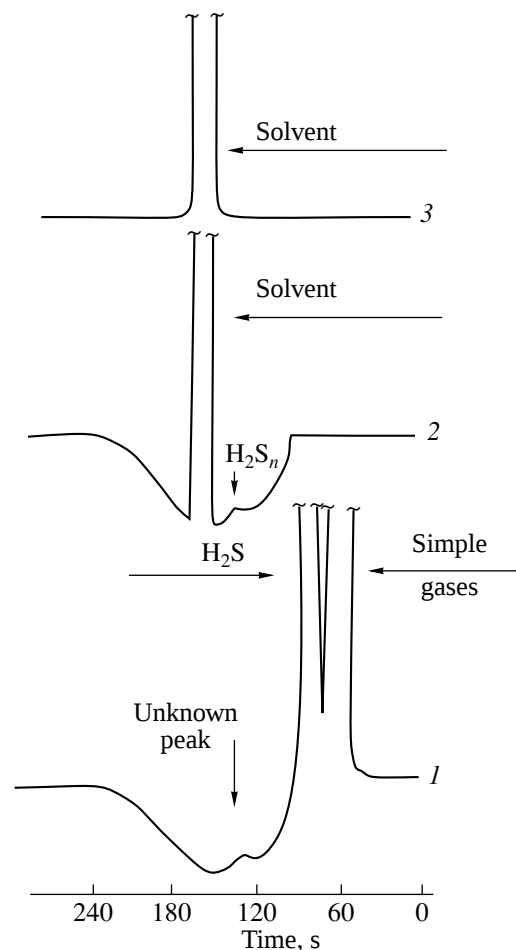
Fig. 5. Chromatograms of (1) the reaction gas mixture, (2) hydrogen polysulfide extracted with diethyl ether, and (3) solvent.
