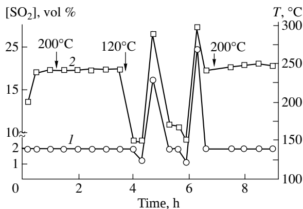
Fig. 3. Plots of the (1) SO_2 concentration and (2) reaction temperature vs. reaction time at an H_2S concentration in the initial gas mixture of 2 vol %, an O_2/H_2S ratio of 5, and a contact time of 0.2 s. The temperature of the initial gas mixture changed during the reaction.
